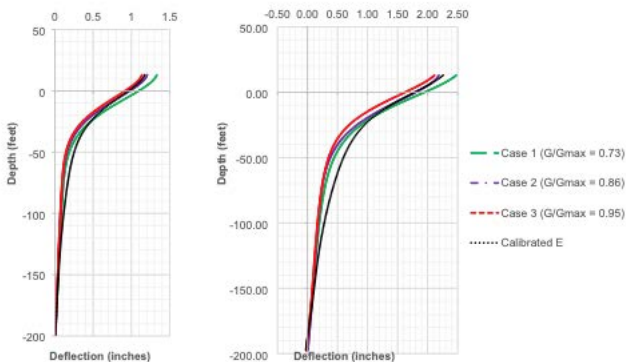
Fig. 12. Reaction Frame Deflection: Left) Rotator, Right) Oscillator
