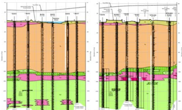
Fig. 3. Site Stratigraphy at Piers 614 Through 618
