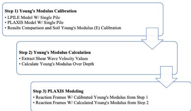
Fig. 7. Methodology to Evaluate Reaction Frame Deflection
