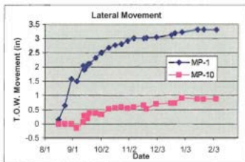
Fig. 11: Horizontal Movement - MP-1 & MP10
