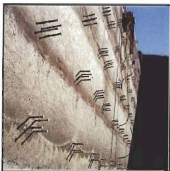
Fig. 3: Soil Nail Matrix
