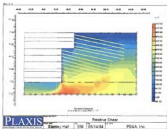
Fig. 13: Relative Shear Stress
