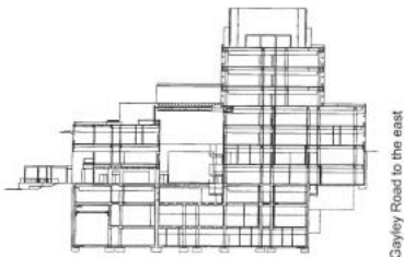
Figure 1: Building Cross-Section
