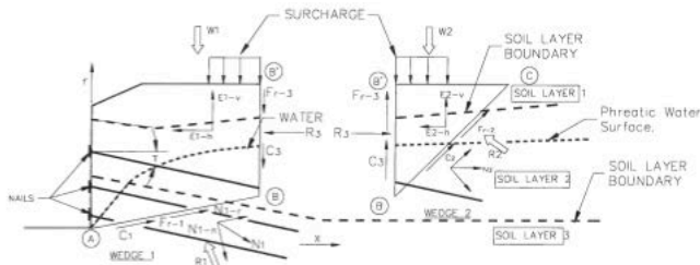
Fig. 6: Freebody Diagram
