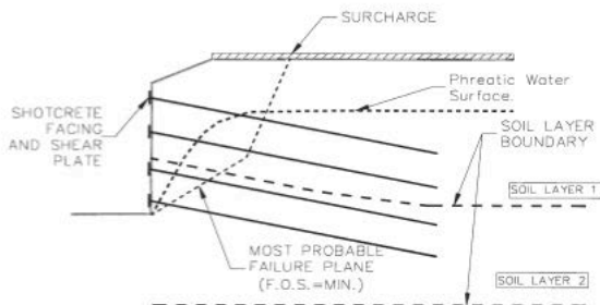
Fig. 4: Typical Soil Nail Wall Section
