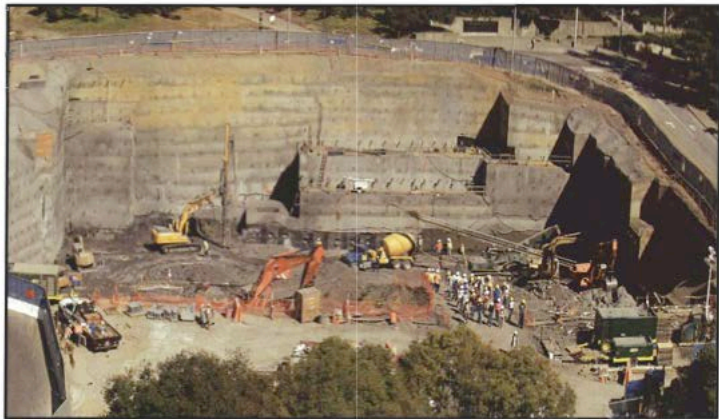
Figure 2: Stanley Hall Excavation, east wall view
