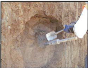
Fig. 10: Recessed Shear Plate
