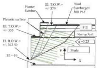
Fig. 8: Wall Model at South-East Corner
